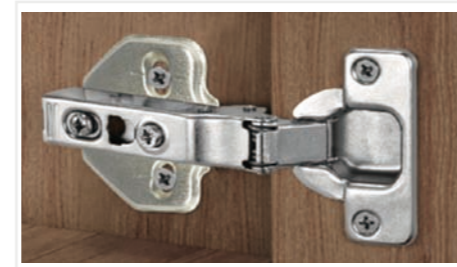
Name Faula Mobilier 110° hinge Code PWWM0051B Notes Applied to full overlay doors and door thickness ≤ 22mm. Soft closing.
