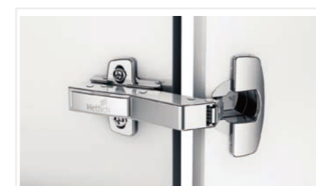
Name Hettich 45° hinge with integrated silent system Code PWWM0046 Notes Applied to pentagonal corner cabinets, full overlay
