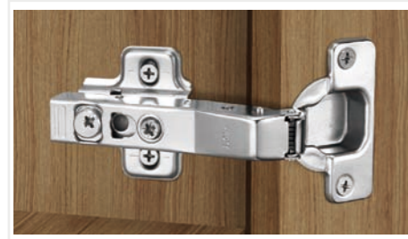
Name Faula Mobilier 45° hinge with integrated silent system Code BWWM0008B Notes Applied to pentagonal corner cabinets.
