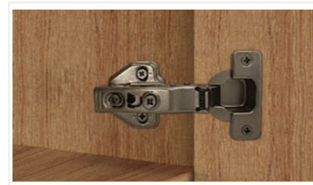
Name Faula Mobilier rebounding hinge Code PWWM0108B Notes Applied to thickened full overlay doors, door thickness ≤ 25mm, matching rebounder.
