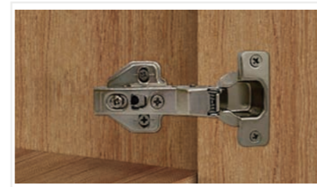
Name Faula Mobilier rebounding hinge Code PWWM0109B Notes Applied to thickened half overlay doors, door thickness ≤ 25mm, matching rebounder.
